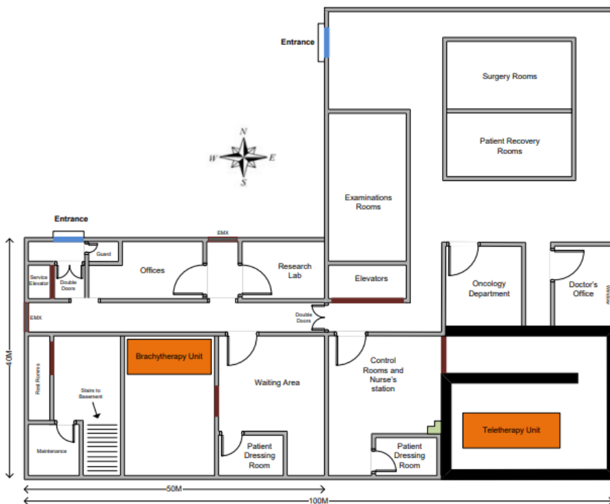
Gambar II.2 Layout Unit Teleterapi X di Rumah Sakit ABC
