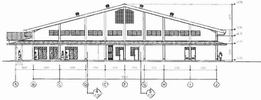
TAMPAK KANAN (VIEW B)
