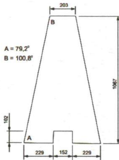
Gambar 6 Single Slope
