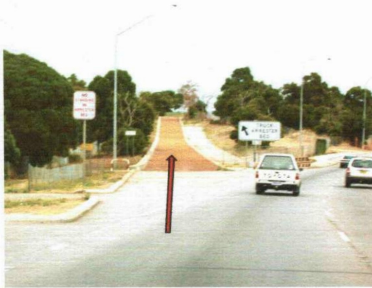
Gambar 71 Landasan Penghenti ( Arrested Bed )
