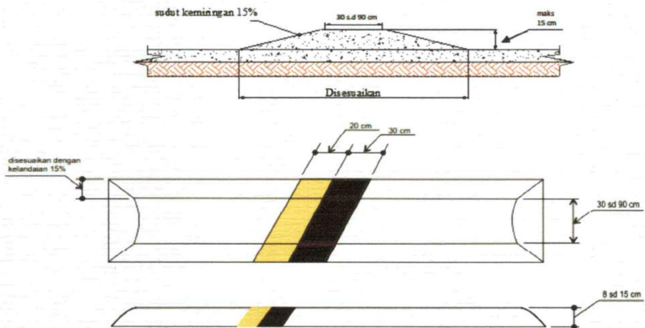
Gambar 2 Speed Hump
