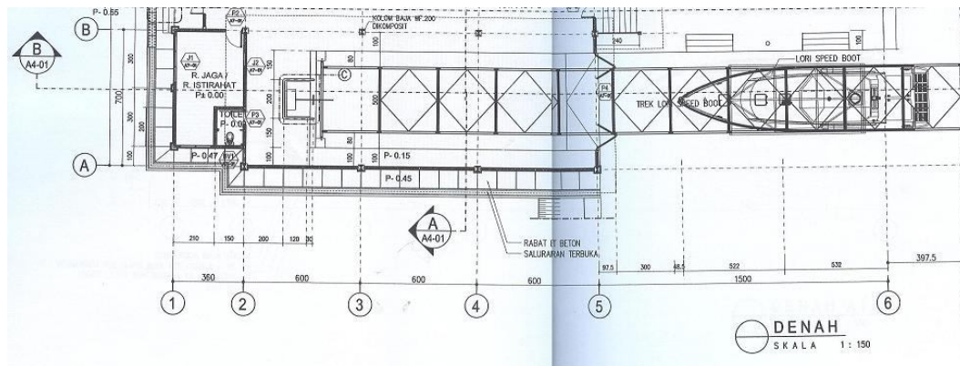
Denah Steiger Speed Boat Pengawasan
