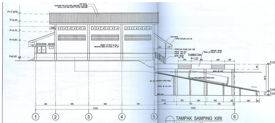
Tampak Samping Steiger Speed Boat Pengawasan
